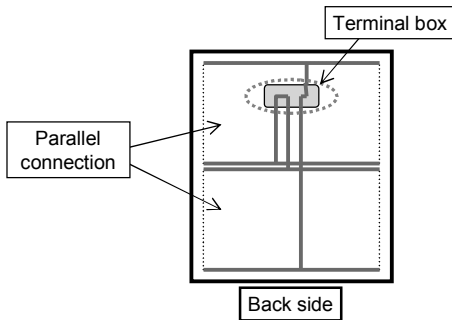
(b) Wiring for module
