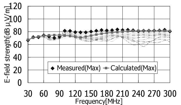
Fig.10 Radiation characteristic of solar battery module
