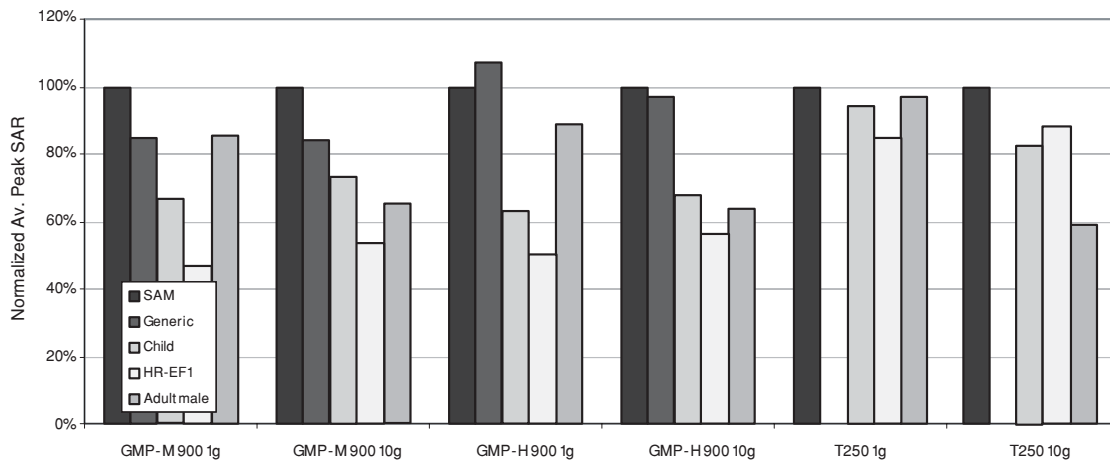
Figure 4: Comparison of the maximum spatial peak SAR obtained by the different phantoms in the two tested positions, whereby all results were normalized to the spatial peak SAR assessed for SAM.
