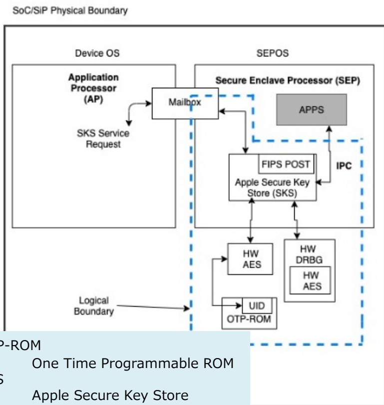
Figure 1: Cryptographic Module Block Diagram
