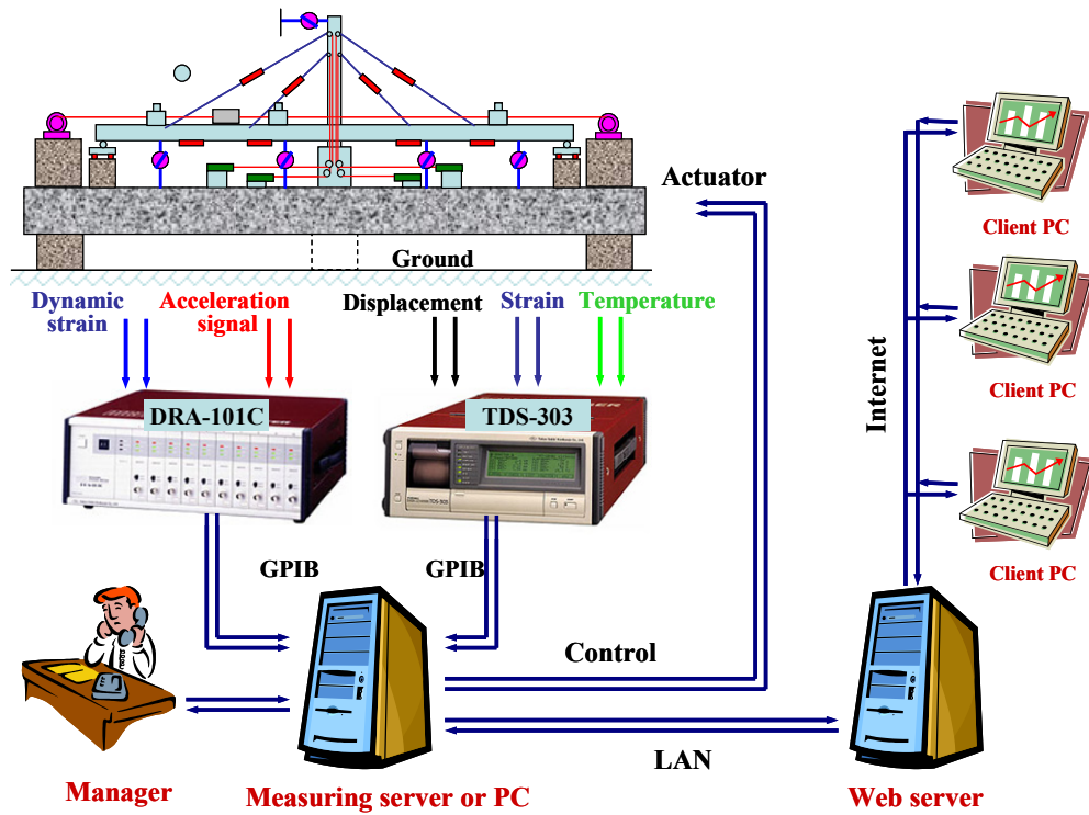
Figure 1 An image of internet remote monitoring system
