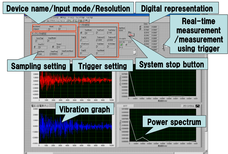
Figure 7 Output screen of vibration monitoring by LabVIEW
