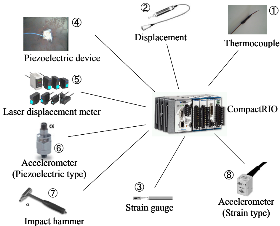
Figure 6 Attachable sensors to CompactRIO
