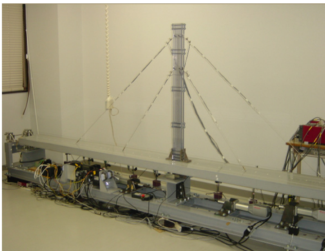
Figure 3 Configuration of para-stressing bridge system
