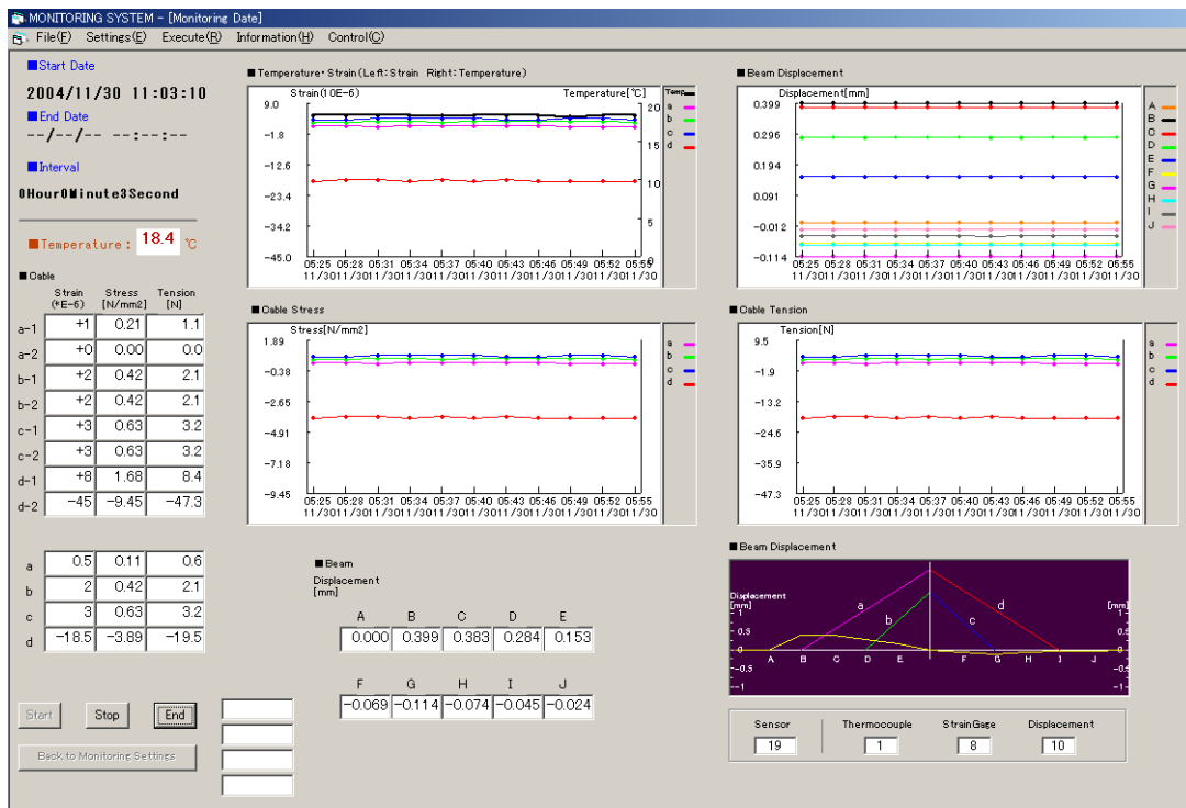
Figure 2 A graphic display of measurement data from the SMS
