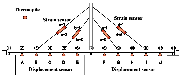
Figure 4 Cable-stayed bridge model with an internet remote monitoring system(IRMS) & para-stressing system
