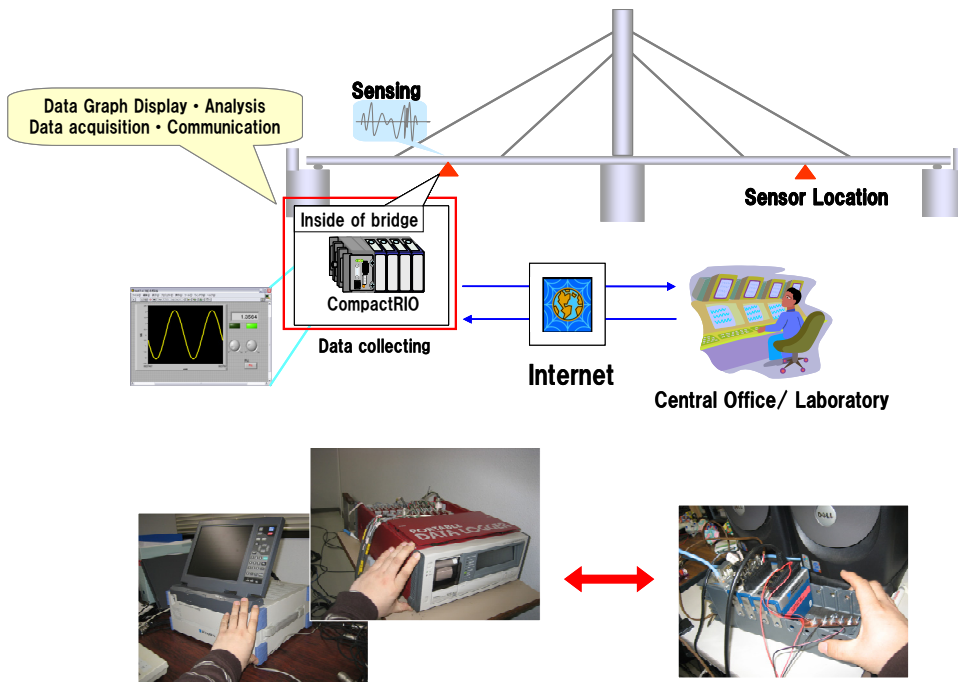
Figure 5 CompactRIO-based data collecting system
