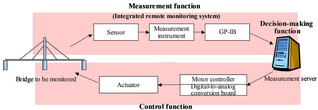
Figure 3 Configuration of para-stressing bridge system
