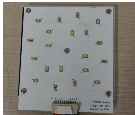
Figure 3. Illumination source consists of 20 LEDs with five kinds of color
