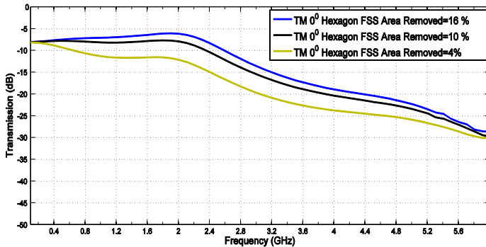
Fig. 10 Simulation transmission results with hexagon FSS for TM polarization with variable aperture width at normal incidence
