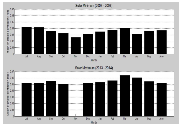
Fig. 2. Comparison of monthly mean phase scintillation \sigma_\phi at low and high solar activity periods. In November 2013, the GISTM receiver had technical problems that caused no data to be obtained for the month.
