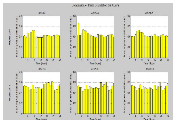
Fig. 3. Comparison of hourly mean \sigma_\phi for three days in August 2007 and August 2013.
