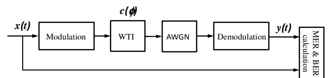
Fig. 1. Channel model used for BER calculation of 16-QAM system with wind turbine interference (WTI) and additive white Gaussian noise (AWGN).
