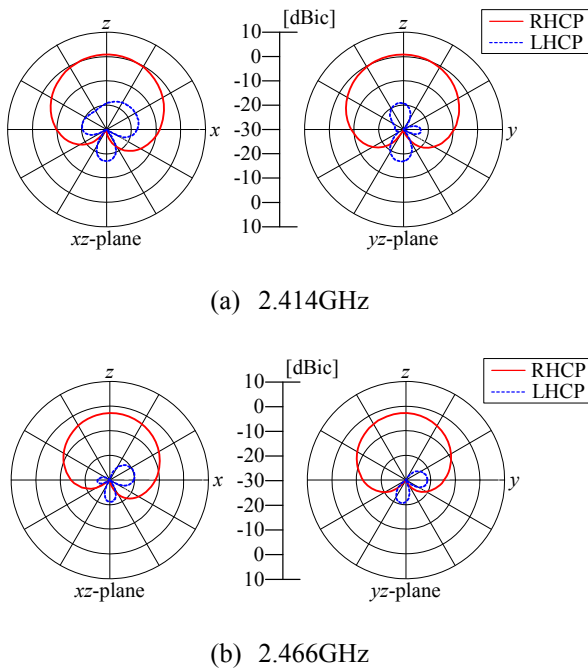
Fig. 3. Simulated radiation patterns.
