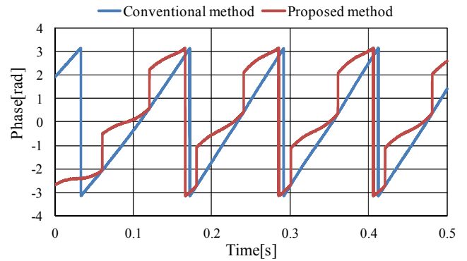
Fig. 5. Phase-Time characteristic
