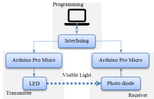
Figure 4. System overview
