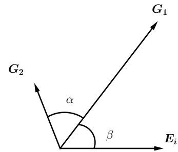
Fig. 1: Two receiving antennas with polarization non-orthogonality and amplitude imbalance in a 2 \times 1 diversity system.
