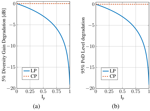
Fig. 2: 1-bitstream degradation of the (a) diversity gain at 5% CDF level, and (b) 95% PoD level, vs. the polarization non-orthogonality factor.
