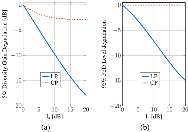
Fig. 3: 1-bitstream degradation of the (a) diversity gain at 5% CDF level, and (b) 95% PoD level, vs. the amplitude imbalance factor.
