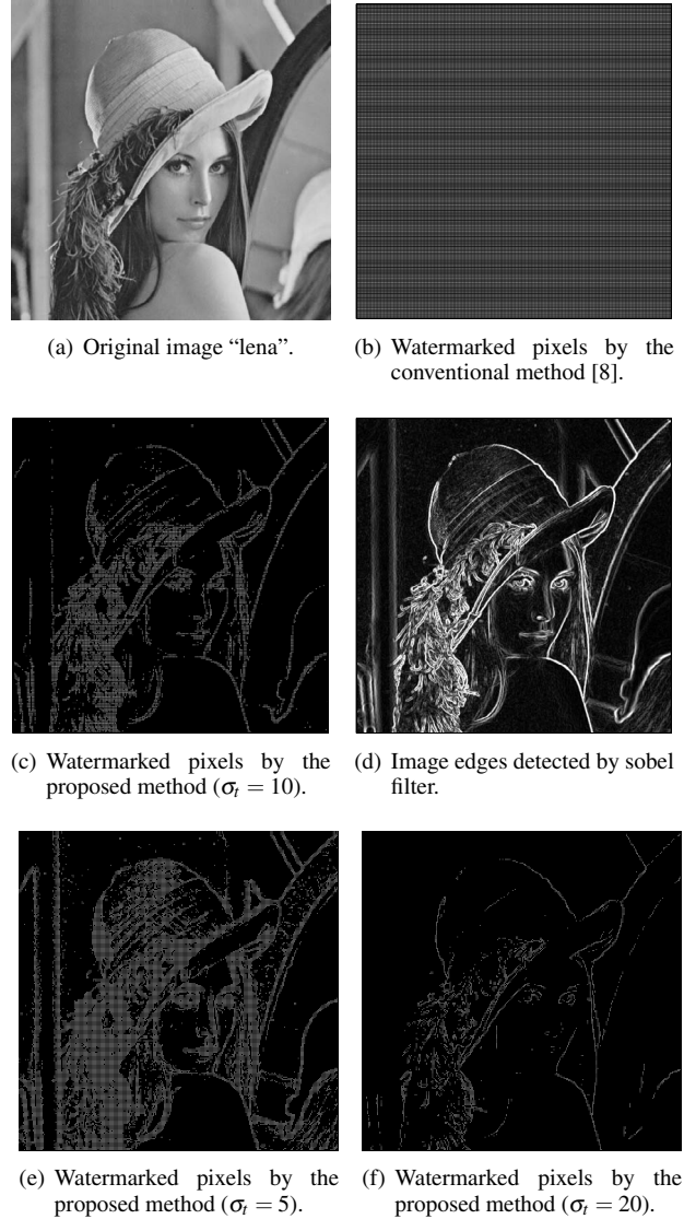
Figure 4. Watermarked pixels by the conventional and proposed method.
