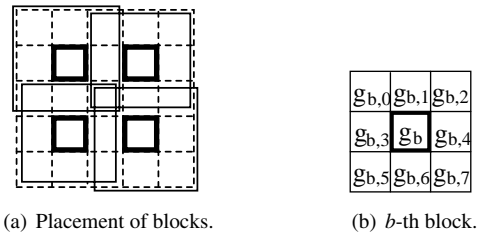
Figure 2. Divided block and its placement.
