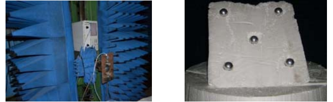
Fig.8. Scanning frame and probe. Fig.9. Real picture of five metallic balls.
