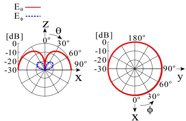
Fig. 10. Radiation pattern for the FAA_{meander} at f_{L-VSWR} = 2.88 GHz, where l_{bent} = 0.375 , N = 3 , and M = 1 mm. (a) In the x-z plane. (b) In the x-y plane.
