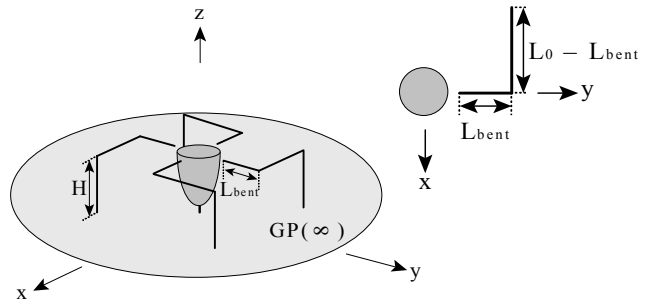
Fig. 6. FAA_{bent} , where the horizontal wires are bent.
