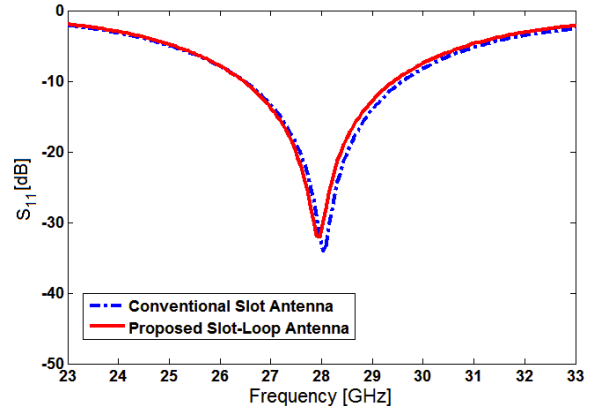
Fig. 5. Simulated S_{11} characteristics of the conventional slot antenna and proposed slot-loop antenna.
