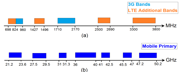
Fig. 1. (a) Frequency bands of 3G and 4G, (b) candidates Bands for 5G in 20-50 GHz (US).
