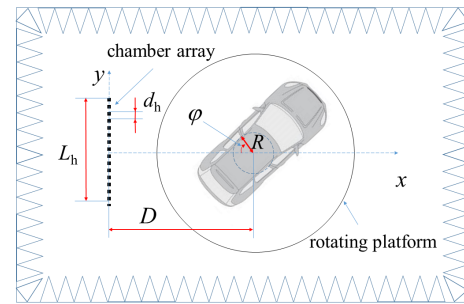
Fig. 1. Schematic representation of RLOS OTA measurement setup geometry in anechoic chamber.
