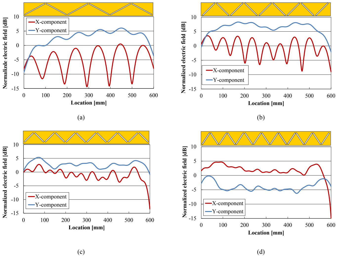
Fig. 5 Normalized electric field of changing the number of slots
