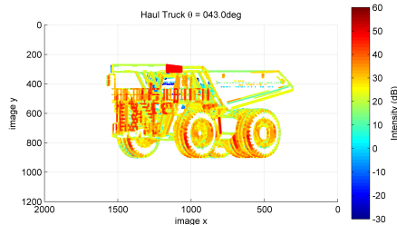
Fig. 5: Simulated response at ( 43^\circ ). Note the significant return from the lip of the bucket.
