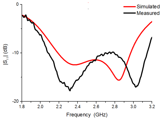
Figure 11- Simulated vs. measured scattering parameters
