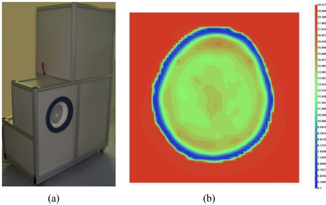
Fig. 1 (a) Overall view of the EMTensor Brain Imaging System Generation 1 (EMT BRIM G1) and (b) MT image of a volunteer's head using the imaging system [12].
