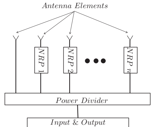
Fig. 6. Diagram for the nonreciprocal antenna array. The group delay of NRP 1 will be designed to achieve the specific phase shifts for all frequencies according the request. And the group delay of NRP n will be n times of the NRP 1.
