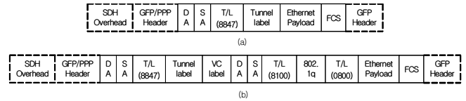
Fig.1. Frame format for (a) premium multimedia service and (b) L2 VPN service
