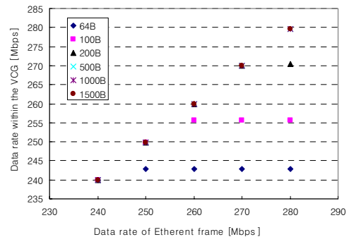
Fig.4. Data rate against Ethernet frame size
