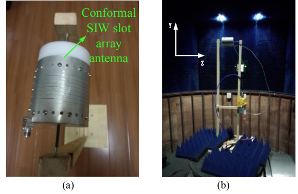
Fig. 4. (a) photograph of the conformal antenna curved on a cylinder with R=34.7 mm, (b) photograph of the measurement setup for measuring its radiation pattern.
