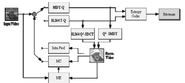
Figure 4. A block diagram of the video encoder based on the MDT
