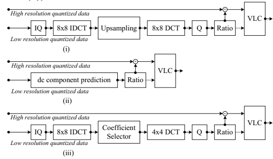
Fig.4 Prediction schemes
