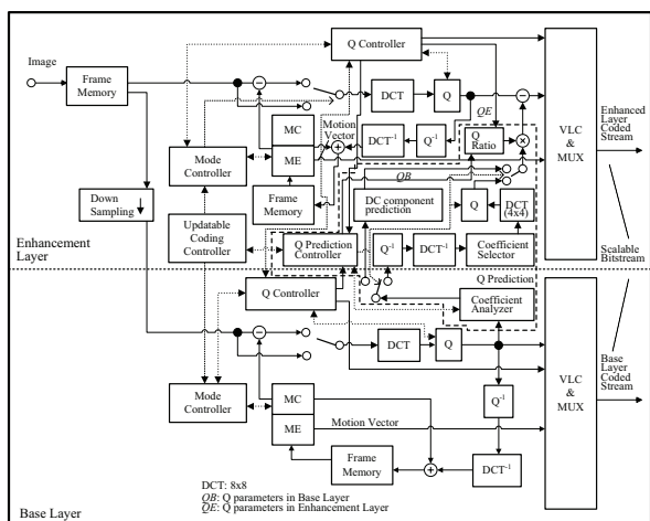
Fig. 5 Adaptive encoder of proposed methods
