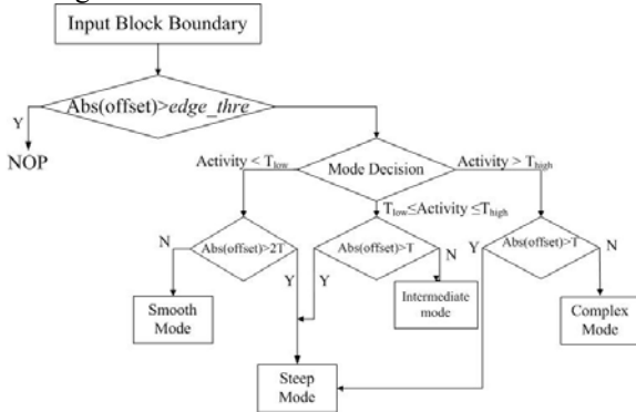
Figure 5. Flowchart of the proposed enhancement algorithm.
