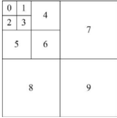
Figure 2. 8 x 8 DCT block taken as ten-subband decomposition.
