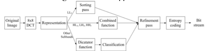
Figure 6(a). Flowchart of the DCT-based-MSPIHT encoder
