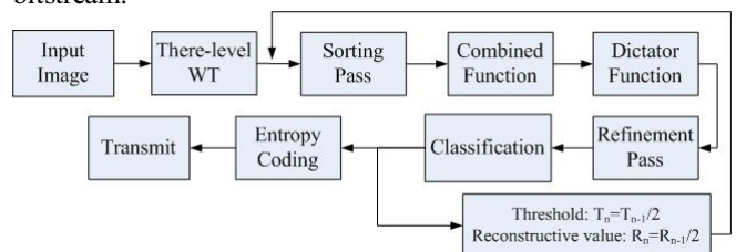
Figure 1. MSPIHT algorithm.
