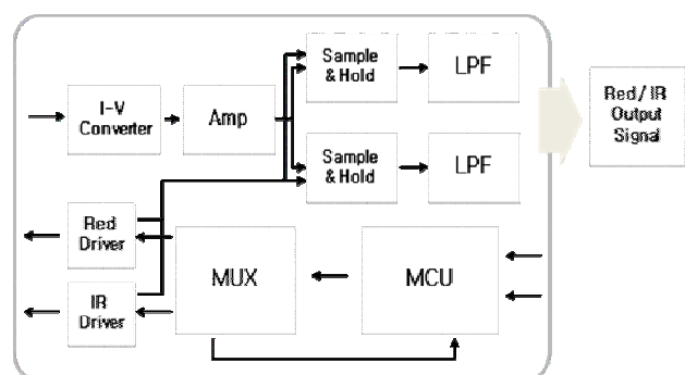
Fig.1. System block diagram of PPG.
