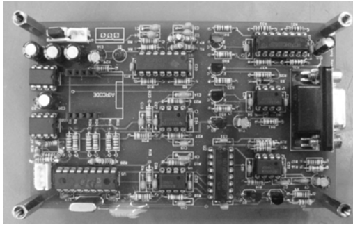
Fig.2. Developed PPG circuit board.
