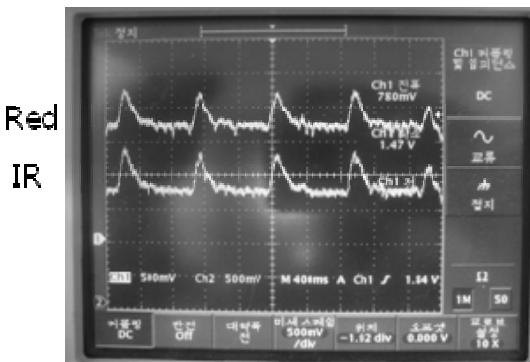
Fig.8. PPG signal measured at '3' in Fig. 5
