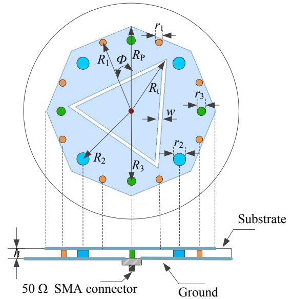
Fig. 1 Configuration of the proposed antenna
