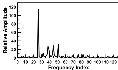
Fig. 5. Measured frequency spectrum of the proposed sensor.
