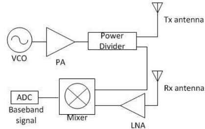
Fig. 1. Architecture of Doppler noncontact vibration-detection radar system
