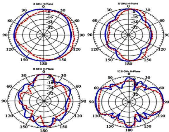
Fig. 3. Radiation pattern of array [A] at 0°
