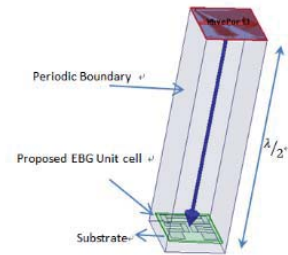
Fig. 2. HFSS reflection phase simulation model.
