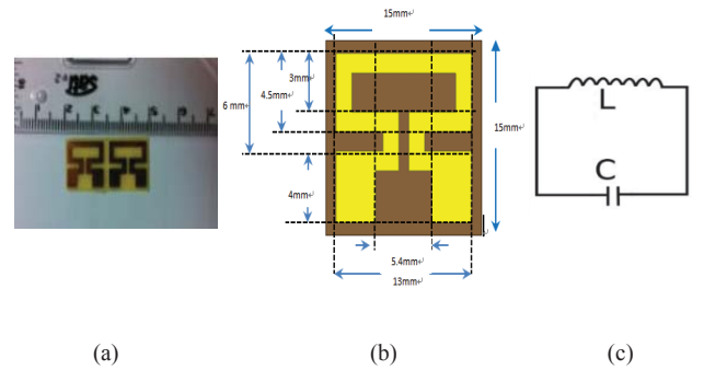
Fig. 1. (a) Proposed planar EBG structure. (b) Dimension of unit cell proposed planar EBG. (c) Equivalent circuit of proposed EBG structures.
