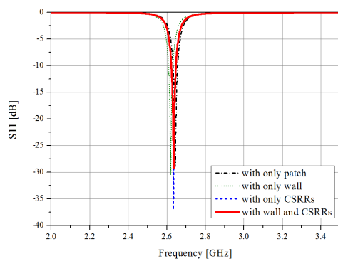
Fig. 4. Return loss result of proposed structure.
