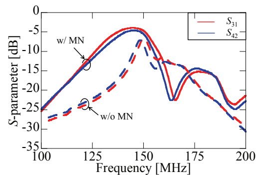
Fig.5 Transmission power
