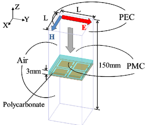
Fig. 2. Analysis model.
