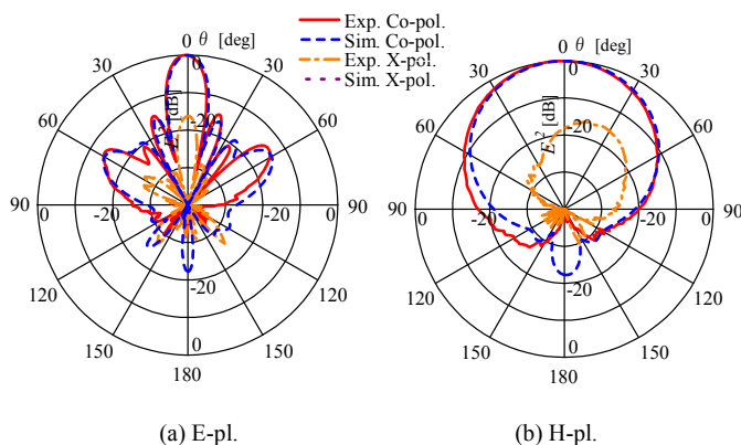
Fig. 3. Radiation patterns.
