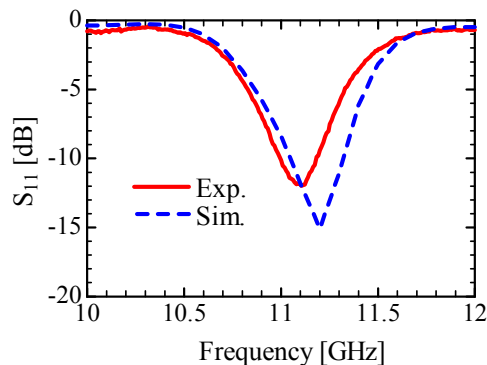
Fig. 2. Reflection characteristics.
