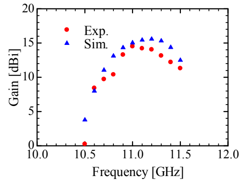
Fig. 4. Gain.
