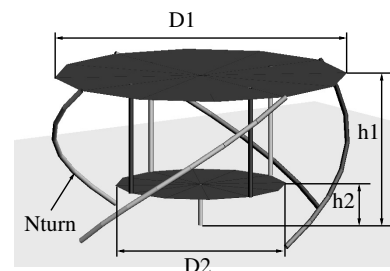
Fig. 1. Monopole antenna with quadrifilar cage (section II): h1 = 5.5\text{cm} , h2 = 1.5\text{cm} , D1 = 12\text{cm} , D2 = 7\text{cm} , Wire diameter 2\text{mm} , N\text{turn} = .25
