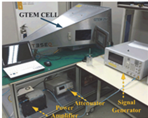
Fig. 2. Measurement set-up
