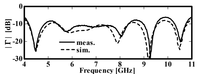
Fig. 2. Matching characteristic.
