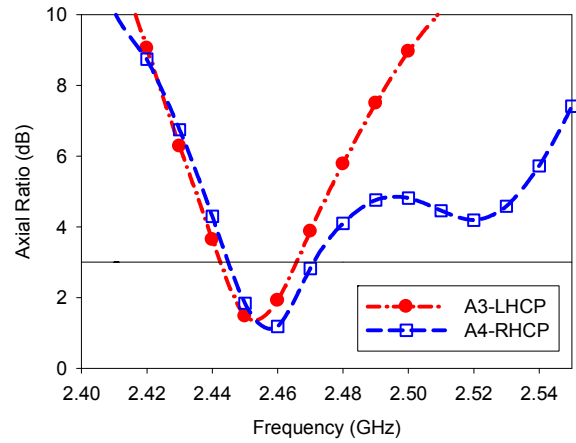
Fig. 3: Simulated axial ratio (dB) for CPs
