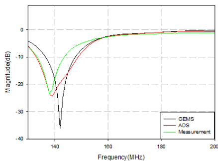
Fig.4 Result of simulated and measured at 140 MHz
