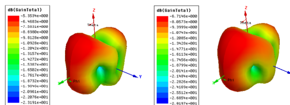
(a) At 4.01GHz of 2nd iteration (b) At 3.86 GHz of 3rd iteration Fig. 4 The radiation of negative gain from different iteration
