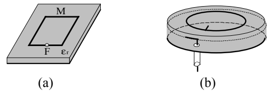
Fig. 1. Loop antennas. (a) LP loop printed on a dielectric substrate. (b) CP loop printed on a dielectric substrate.
