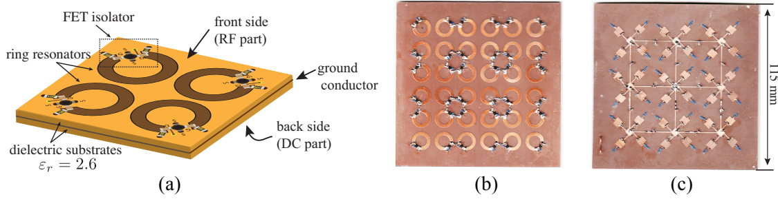
Fig. 3 Proposed PEMC metamaterial surface consisting of non-reciprocal traveling-wave ring resonators. (a) Unit-cell, consisting of 4 gyro-ring resonators. (b) Prototype front side. (c) Prototype backside.
