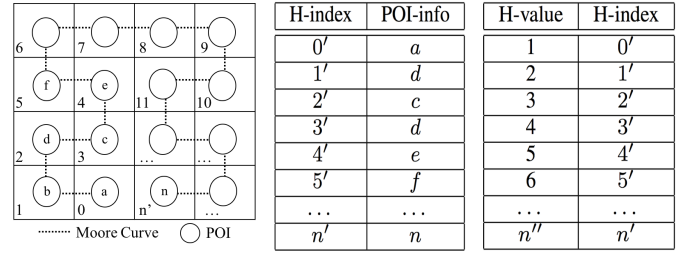
(a) Moore Curve on Grid
