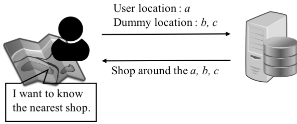
Fig. 1: Example of Dummy-based LBS
