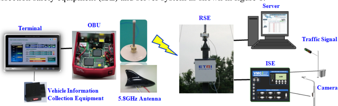
Figure 1: WAVE based vehicular communication system
