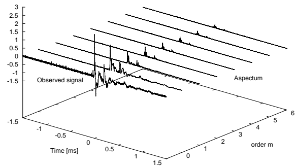
Figure 2 Observed signals and aspectum. (negative CG discharges)
