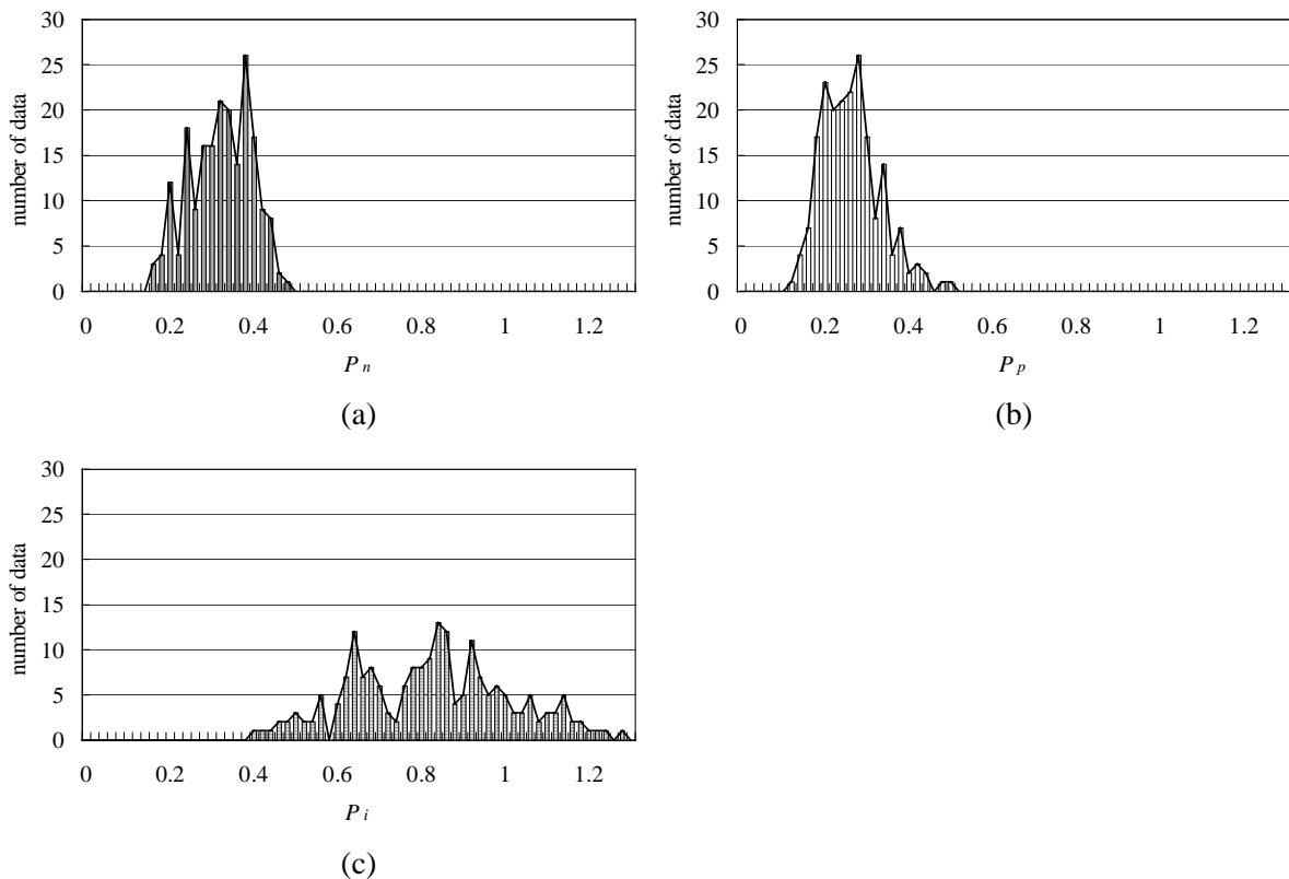
Figure 3 P versus number of data. (a) negative CG discharges case ( P_n ), (b) positive CG discharges case ( P_p ) and (c) IC discharges case ( P_i )
