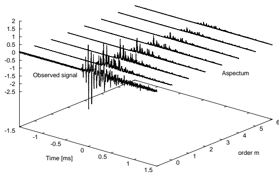
Figure 1 Observed signals and aspectum. (IC discharges)
