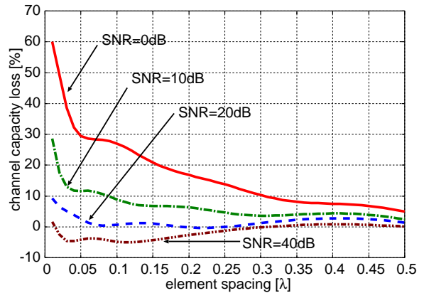
Figure 2: channel capacity loss versus element spacing
