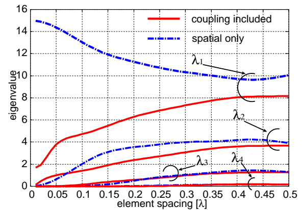
Figure 4: eigenvalue versus element spacing
