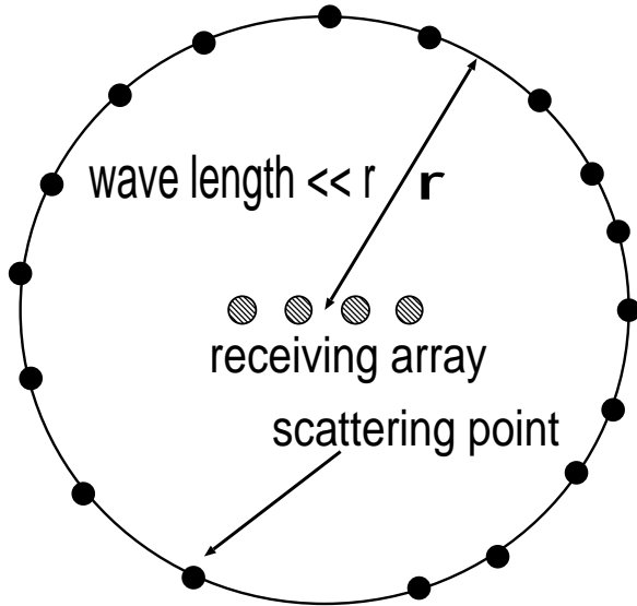
Figure 1: Rayleigh fading environment model
