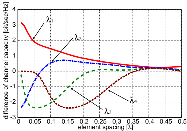
Figure 5: difference of channel capacity at SNR=40dB
