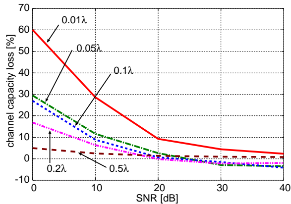
Figure 3: channel capacity loss versus SNR
