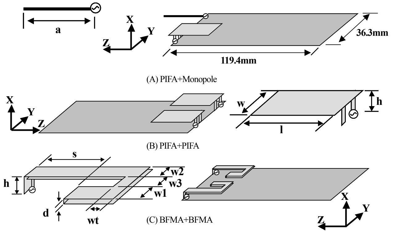
Fig. 1 Antenna configuration
