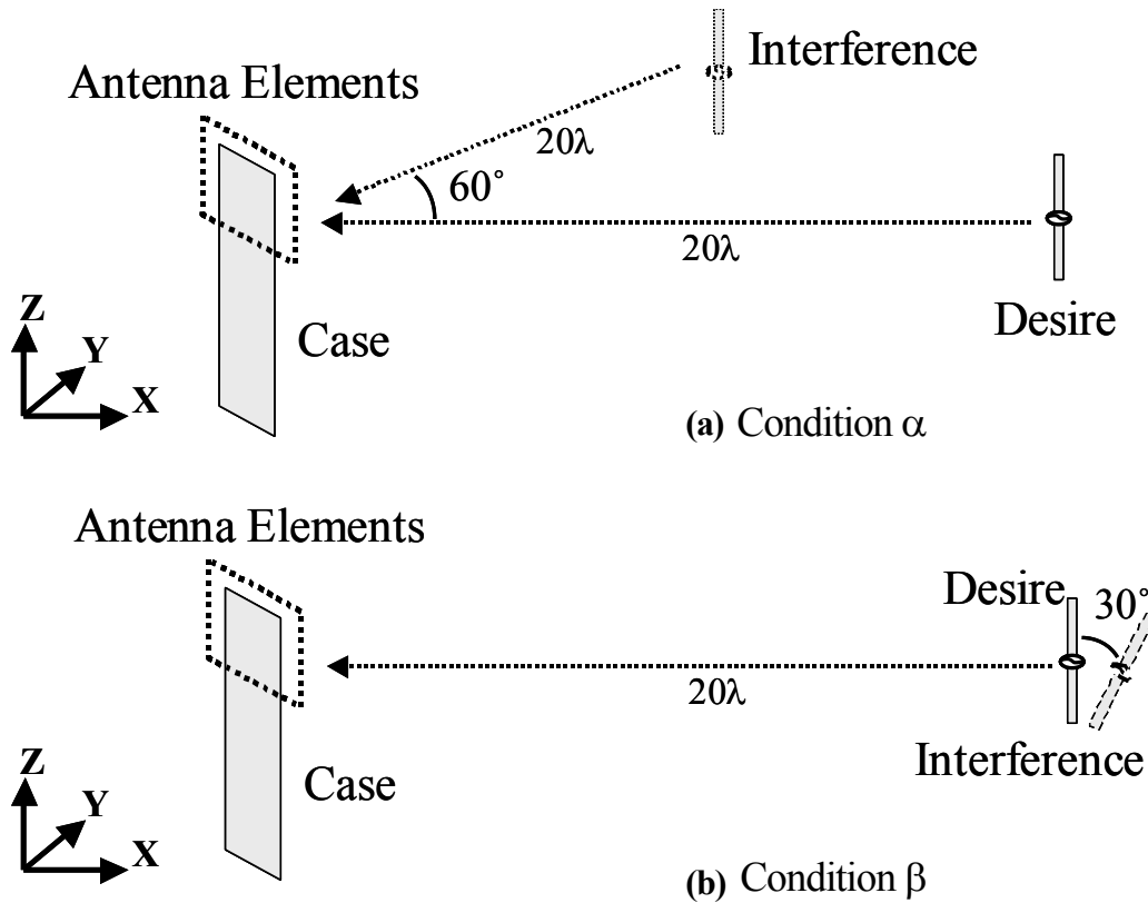
Fig. 2 Simulation model
